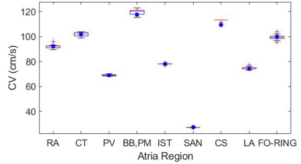
Figure 1 Boxplot showing the variability in conduction velocity across 10 different heterogeneous tissue samples for each atrial region. The blue dot for each region represents the CV for the equivalent homogeneous atrial tissue.
