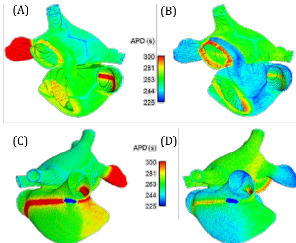
Figure 3 APD maps of the regionally homogeneous atria (A, C) and heterogeneous atria (B, D).
