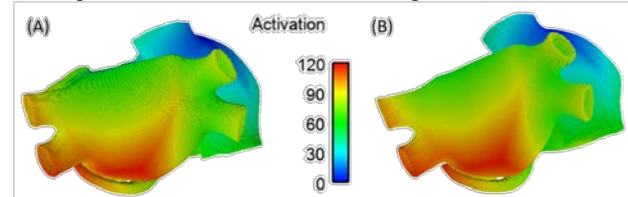
Figure 2 Activation maps for the regionally homogeneous atria (A) and heterogeneous atria (B). The scale shown in the middle of the figure applies to both A and B with activation times ranging from 0ms to 120ms.
