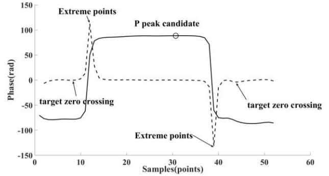
Figure 4. An example of zero crossing detection. The solid line stands for the transformed P region signal while the dotted line represents its first-order difference series.
