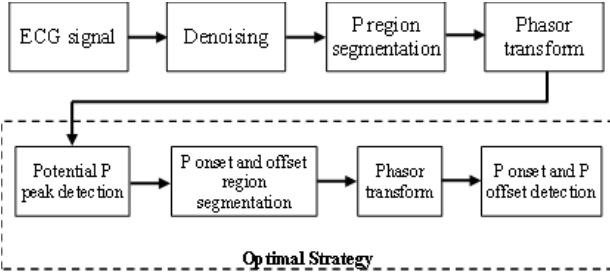
Figure 1. The block diagram of the proposed method
