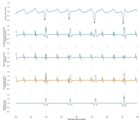
Figure 1. Example of ventricular far-field removal with, from top to bottom, ECG lead V1 with R peaks, original CS dipole signal, reconstructed signal, superposition of the two, difference of the two.
