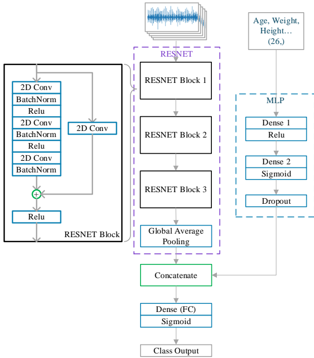
Figure 2. The composition about Murmur classifier.
