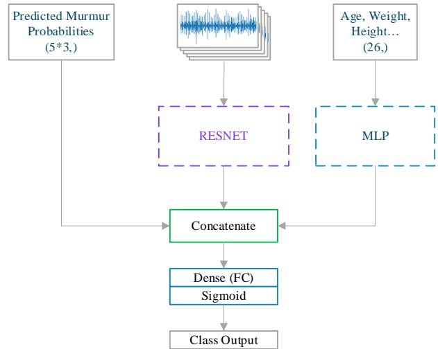
Figure 3. The outcome classifier is concatenate by RESNET blocks and MLP and the predicted values of 5 trained murmur classifiers, then do 2 classifications.
