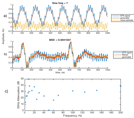
Figure 4. Results before and after applying the combined denoising approach, 4a) reference sine wave and noise estimate; b) ECG signal before/after filtering; c) results of 50 Hz attenuation when testing a range of sine waves with frequencies ranging from 1 to 200 Hz.
