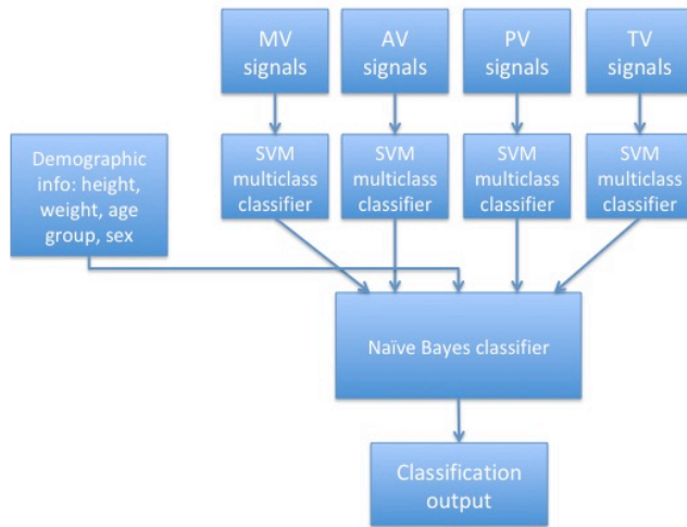
Figure 3. Algorithmic approach to the two Challenge classification tasks. Four signals (at most) are input into four separate SVMs; the outputs of the SVMs and the demographic info are fed into a naïve Bayes classifier to produce the final classification output.
