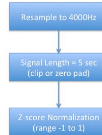
Figure 2. Pre-processing steps applied on the input signals prior to classification.
