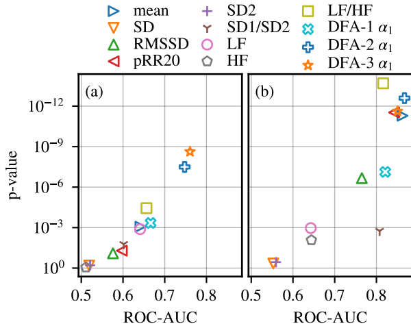
Figure 2. Welch's- t test p -values versus ROC-AUC for different HRV measures. Comparison between healthy and LQTS without (a) and with (b) beta blocker therapy.
