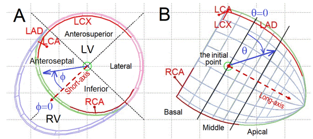
Figure 2. A: The short-axis view the wall segments. B: The long-axis view the regions. RCA, LCA, LAD, and LCX are the coronary arteries
