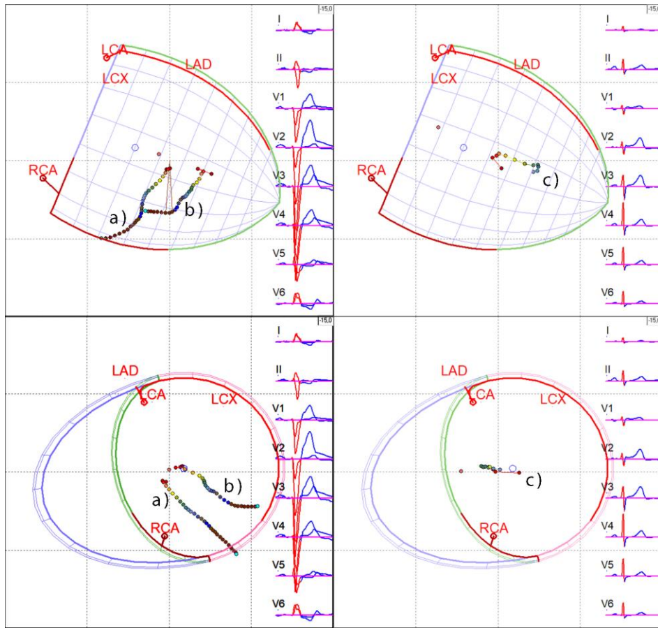
Figure 3.: ED trajectories samples in: a) and b) subjects with LBBB, c) healthy subject
