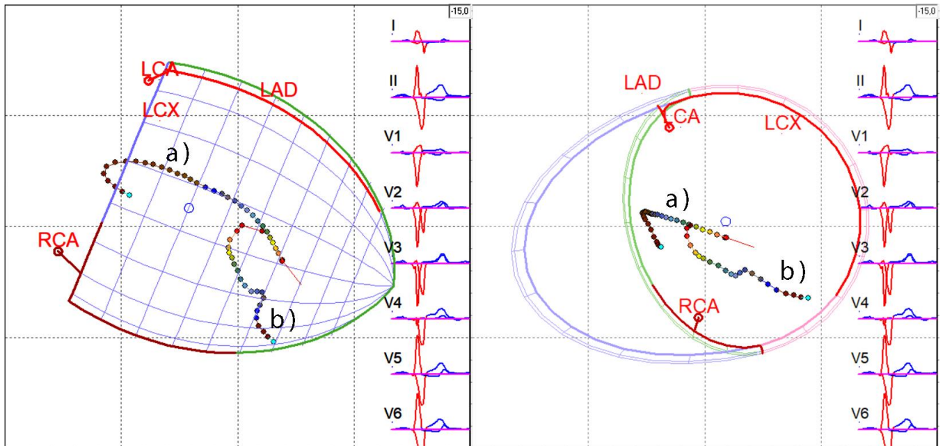
Figure 4.: Representative ED trajectories in two subject from the analysed group; a) BiV pacing, b) CSP pacing
