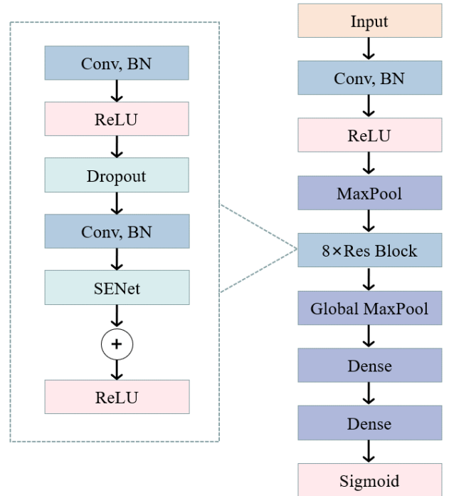
Figure 5. The CNN network architecture used in method two.
