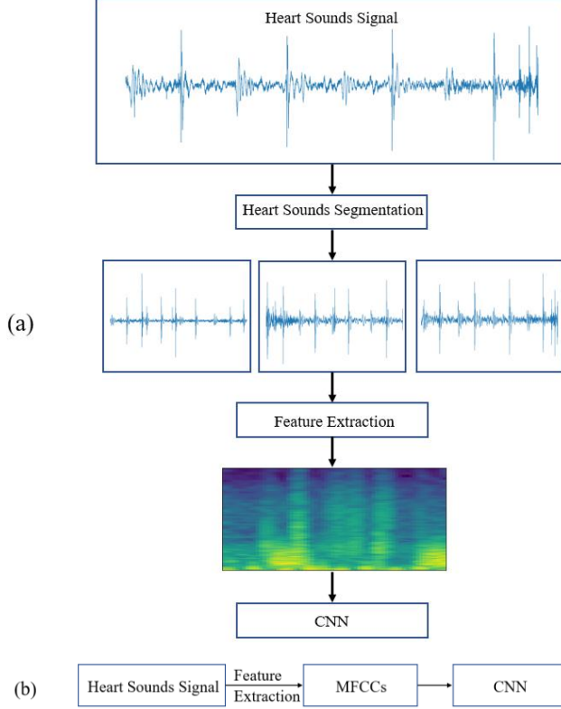
Figure 1. The system-level flow diagram of the proposed methods, (a) denotes method one, and (b) denotes method two.
