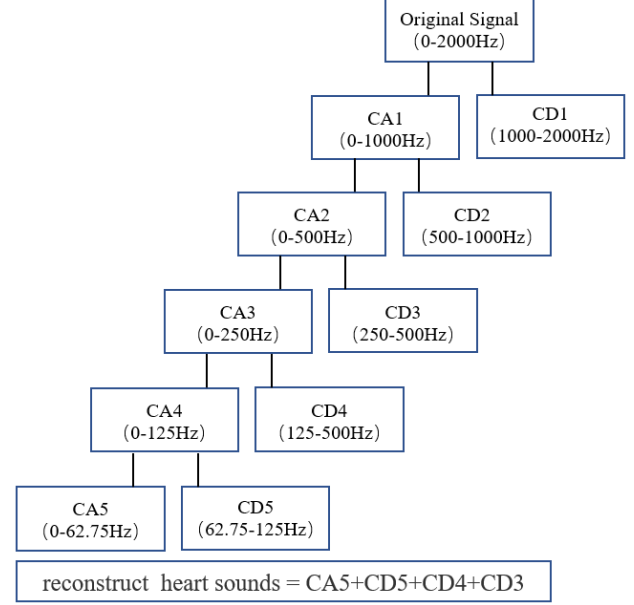
Figure 2. The framework of the corresponding heart sounds signal wavelet denoising algorithm.
