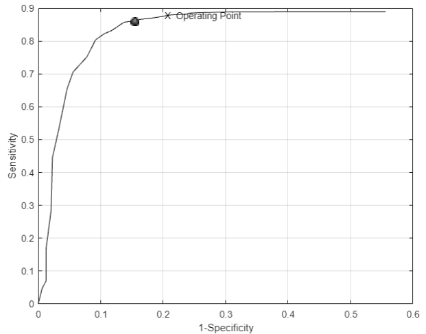
Figure 5: ROC curve assessing the accuracy of AF detection on iOS platforms. x represents the operating point using Android thresholds, while ● represents a potential alternative operating point.
