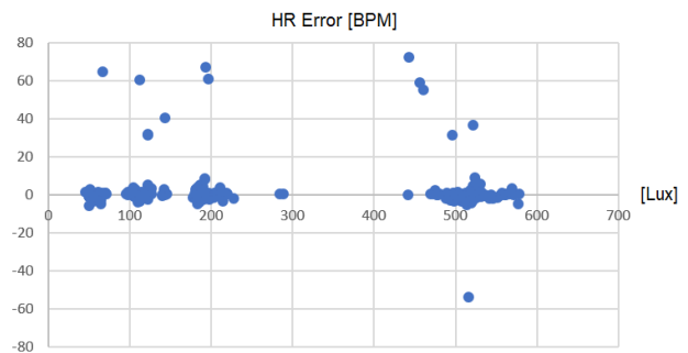
Figure 4: provides the HR accuracy across ambient illumination levels varying from 50 to 500 lux.
