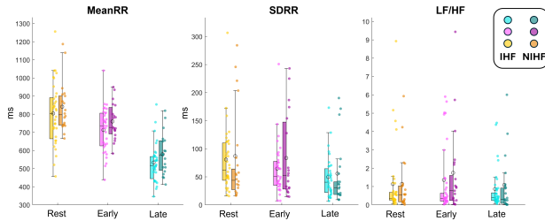
Figure 1. Time- and frequency-domain HRV parameters computed for IHF and NIHF patients at Rest, Early and Late exercise phases. No statistically significant differences were outlined.
