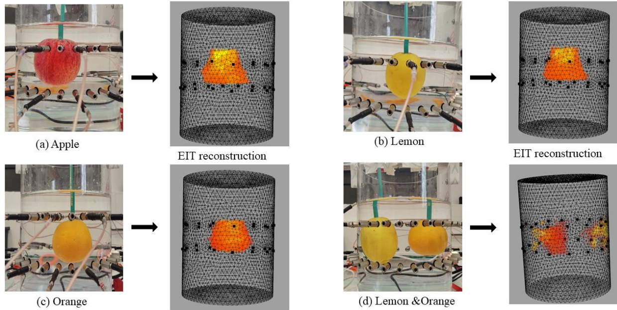
Figure1. EIT results for fruit objects inside a cylindrical imaging tank. The experimental setups (left) show different fruit positions and configurations, while the corresponding reconstructed images (right) display the conductivity distribution.
