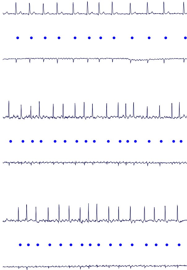
Figure 2. Examples from the AF Termination Challenge Database. The three panels show the final 10 seconds of each of records n02 (top), s02 (center), and t02 (bottom). Annotations between the two ECG signals from each record mark the locations of the QRS complexes. Contrast the atrial activity in the upper panel (sustained AF) with that in the other two panels (PAF).
