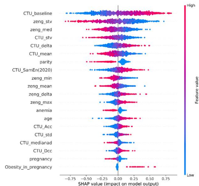
Figure 2. Shapley value importance ranking of Voting Classifier (the top 20 features)
