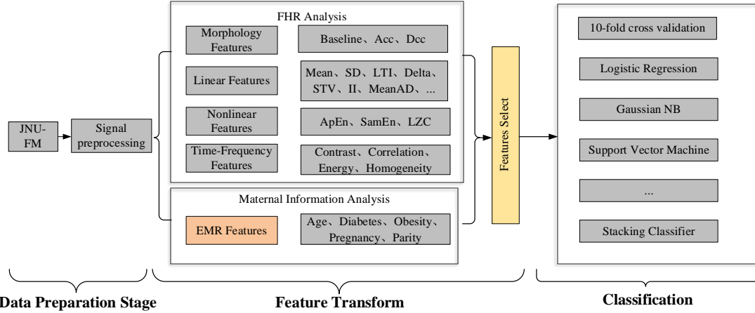
Figure 1. Procedure of the Delivery Mode Prediction (including data preparation, feature transform and classification)
