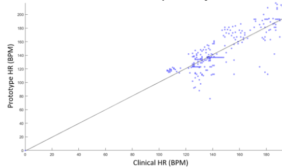
Figure 3. Prototype and Clinical HR Correlation graph for without motion datapoints (n = 284).
