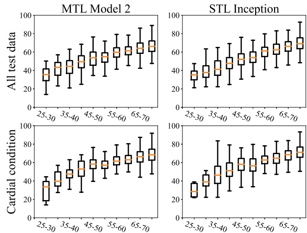
Figure 2. Distribution of age predictions in different age groups on PTB-XL. Higher variance is particularly prevalent in the STL model on cases with cardiac conditions.
