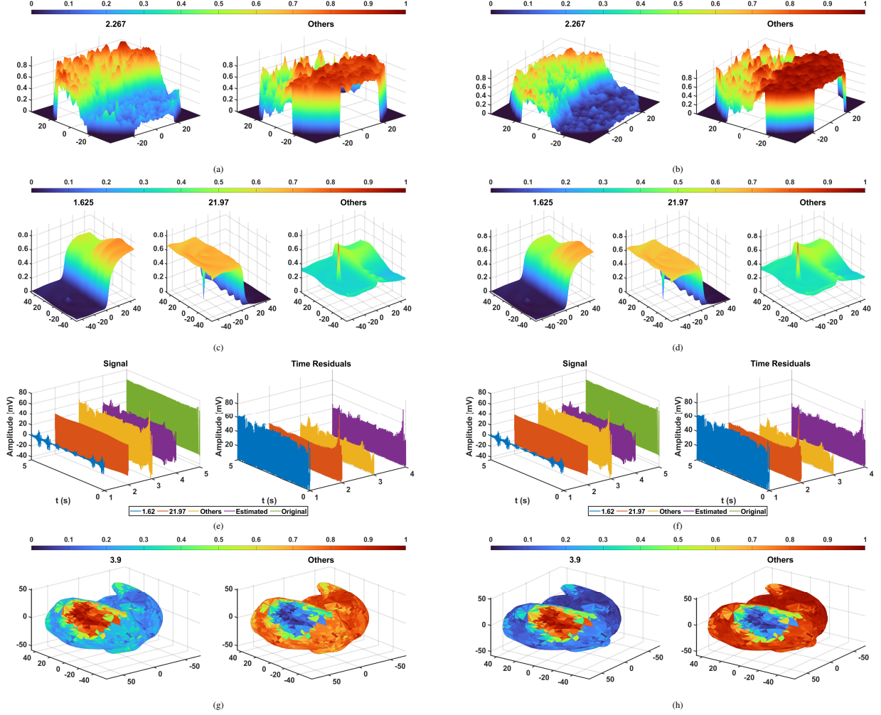
Figure 2. Frequency maps computed using LS and ENR methods across various cases. LS and ENR frequency maps are presented in (a) and (b) for the optical mapping case and in (c) and (d) for the planar cardiac tissue simulation case. The upper panel of (e) and (f) represents the signal estimation for selected frequencies in blue and orange, the signal for remaining frequencies in yellow, the combined estimated signal in purple, and the original signal in green, applicable to both LS and ENR methods. The lower panel of (e) and (f) showcases residuals for the estimated signal of selected frequencies in blue and orange, residuals computed with the remaining frequencies in yellow, and residuals for the estimated signal created by combining the selected frequencies. Finally, (g) and (h) display the frequency maps for 3D fibrotic atria simulation registration computed by LS and ENR, respectively.
