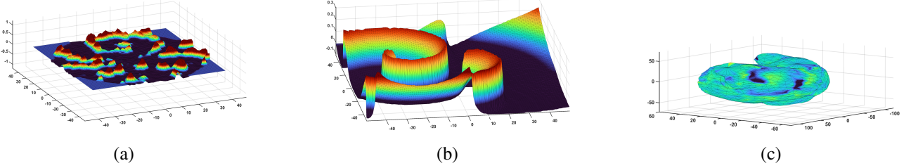
Figure 1. Rotor regions for each presented case: (a) Optical map of rat ventricular myocardium; (b) 2D simulation depicting a rotor; (c) 3D simulation exhibiting fibrosis and an AF focus in the left atrium.
