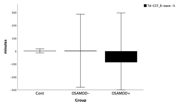
Fig. 3 Time delay (Td) of the \delta -wave from the changes in \lambda .
