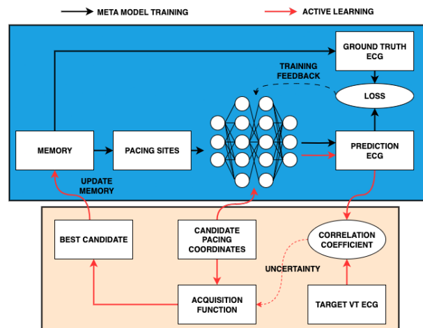
Figure 1. Block Diagram of the Proposed Method
